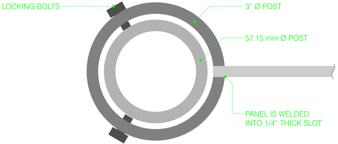
PLAN VIEW 1:10 SCALE
